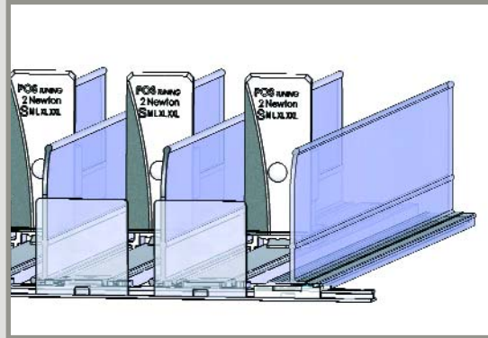
End divider to cap and finalize the end of the shelf compartment.
